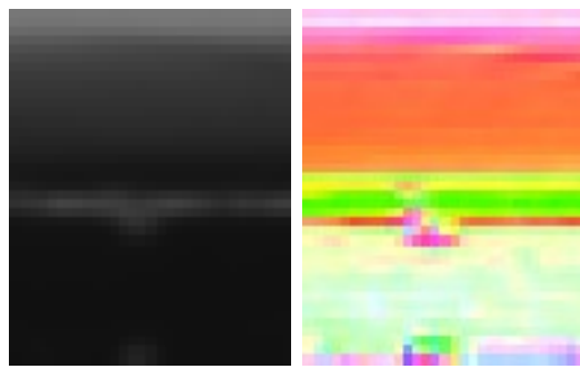
Bilinear
