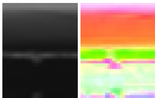
RI (non-edge-aware)
