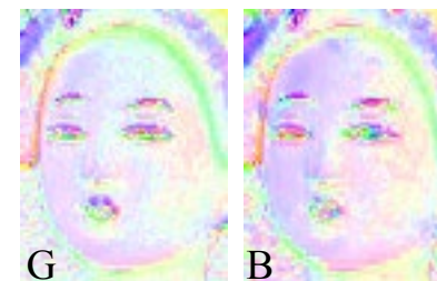
RI | ICPC
