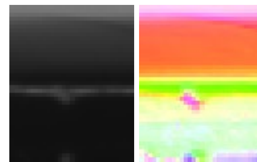
Ground truth
